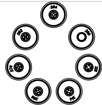
Orifice inserts for brew basket 0.094 is factory installed
