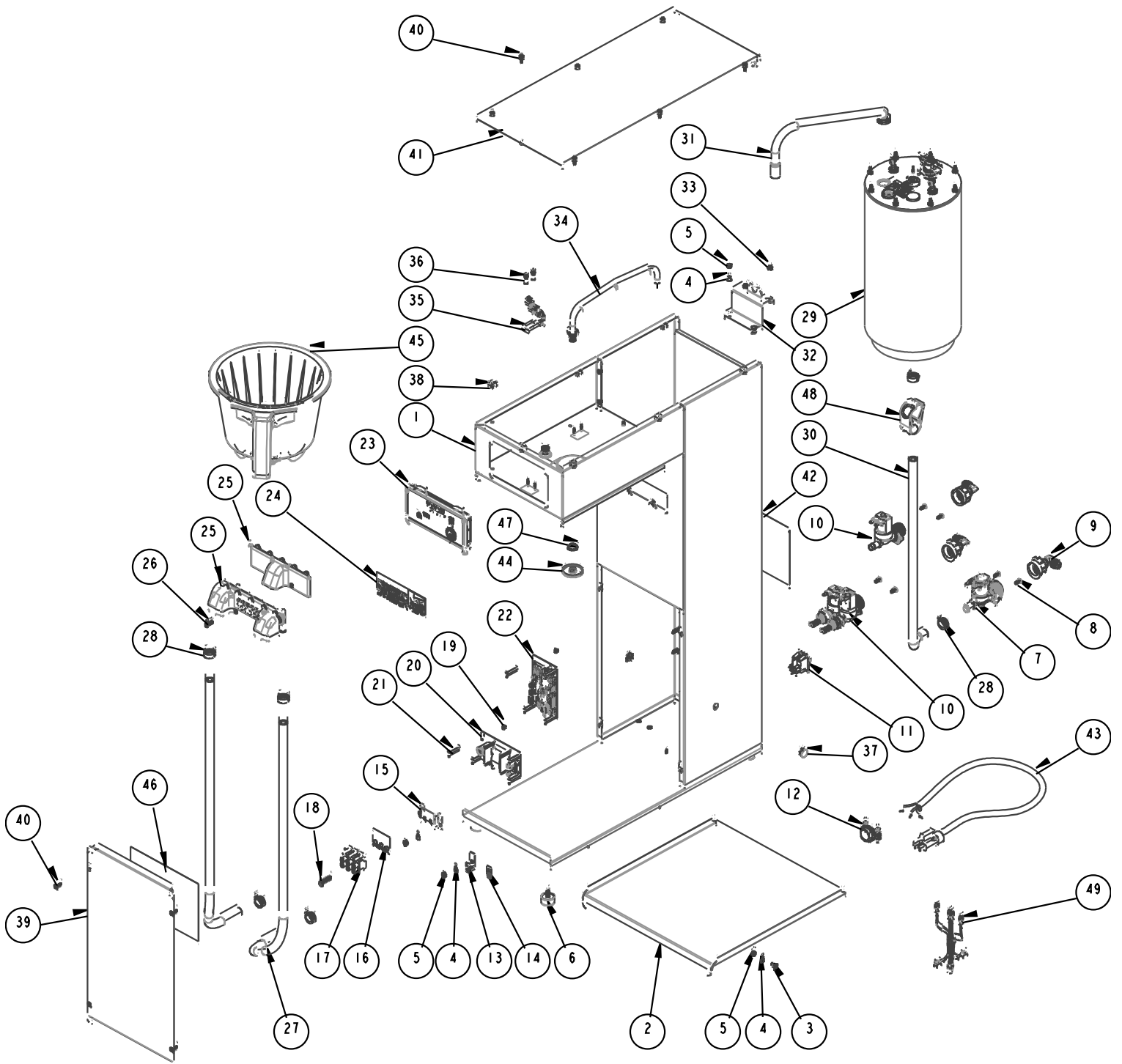
Drawing 1101.00515.00
